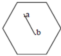
Convex Polygon
